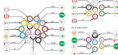
PIN DIAGRAM Adapter 24V
